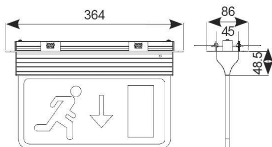
Semi Recessed
